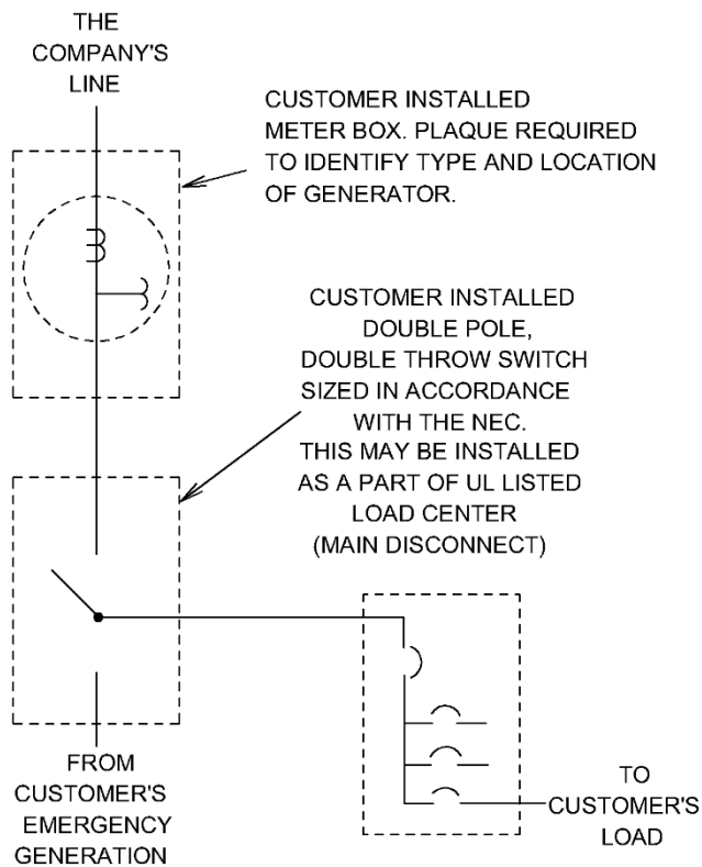
DOUBLE THROW SWITCH "FULL LOAD"
